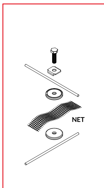
QUBO, PRISMA AND ZEPHIRO SCREWS
